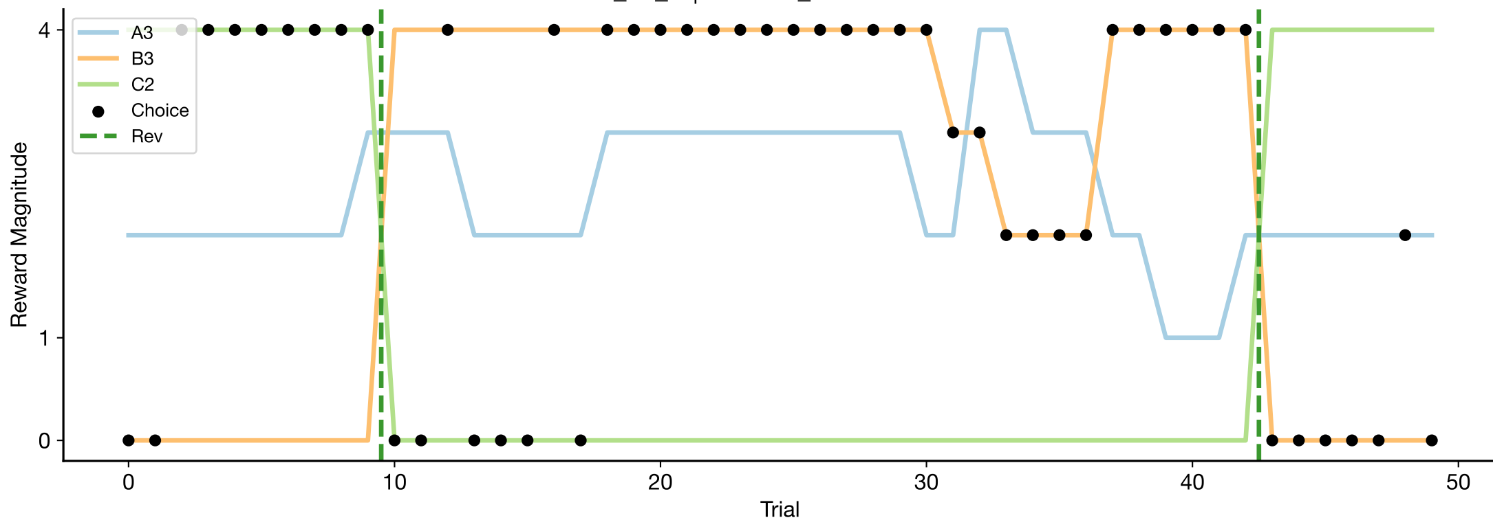
MY_71_R | ses-164_date-20260616
